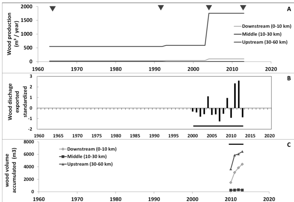
Figure 48. Large wood dynamics trajectory of Saint-Jean River over the period 1963-2013 for the three geomorphological unit's area. (Triangles represent aeriels and satellites imagery use for analysis and black lines represent an annual survey).
